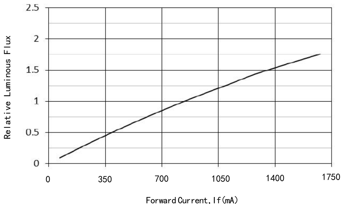
Forward Current vs. Relative Luminous Flux ( T_c = 25^\circ\text{C} )
